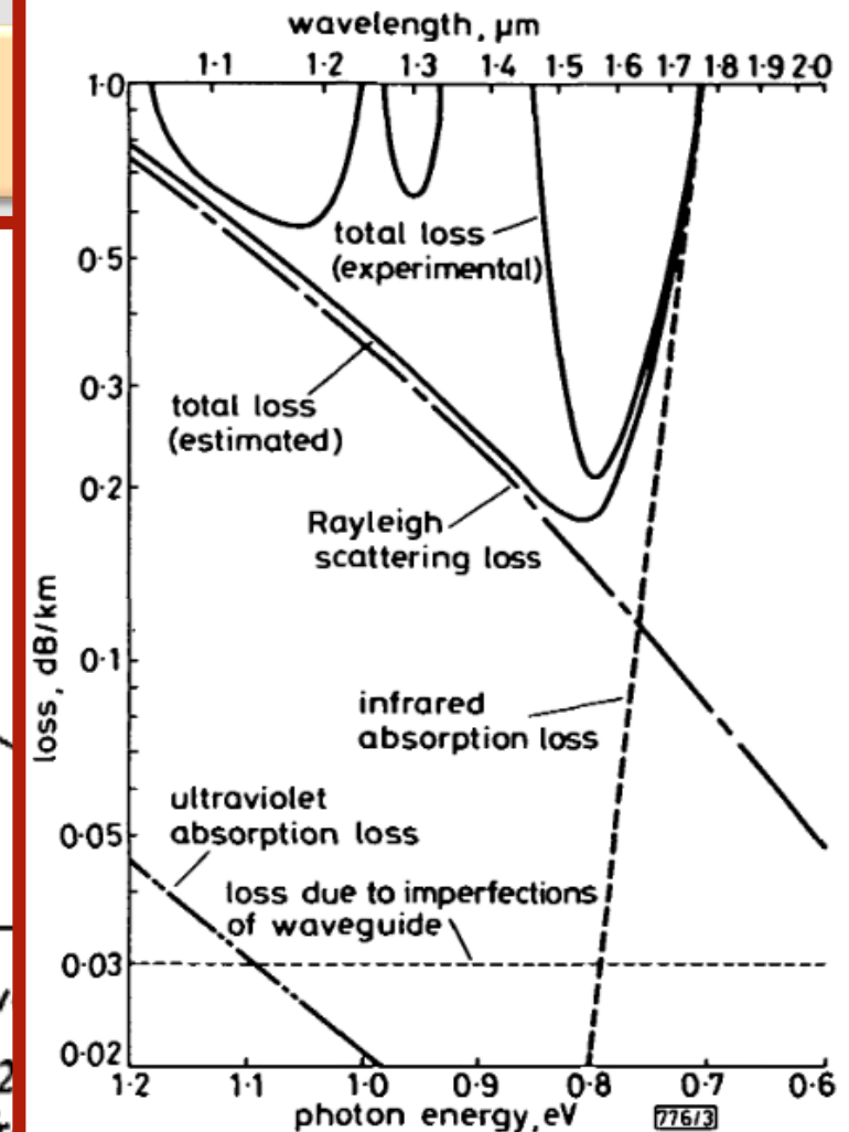
Fig. 3 Transmission-loss mechanism in the optical fibre discussed
