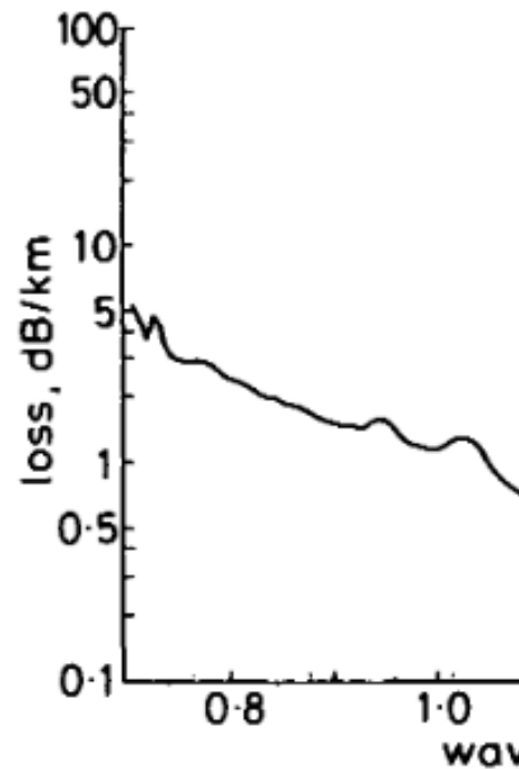
Fig. 1 Spectral loss of 2.2 core diameter, 0.0028 refracting and 1.1 \mu\text{m} cutoff waveguide
